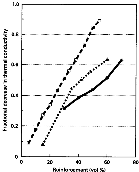
Figure 17 Variation of fractional decrease in thermal conductivity with reinforcement volume fraction of various composites made by the coated filler method. (□) Cu/SiC w ; (Δ) Cu/TiB 2 ; (○) Cu/Mo.
