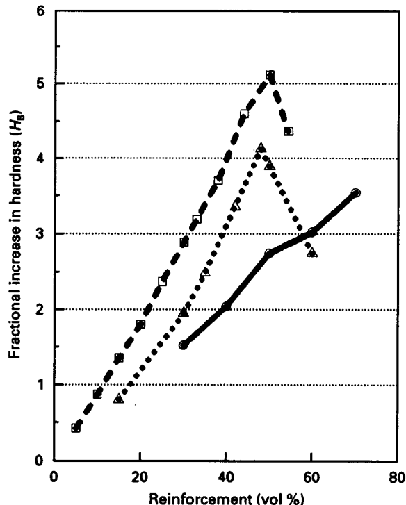
Figure 15 Variation of fractional increase in hardness with reinforcement volume fraction of various composites made by the coated filler method. (□) Cu/SiC w ; (Δ) Cu/TiB 2 ; (○) Cu/Mo.
