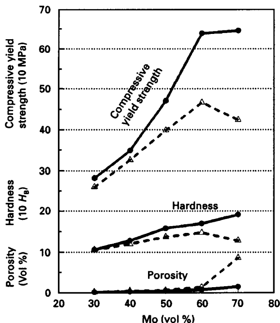
Figure 1 Variation of porosity, hardness and compressive yield strength with Mo particle volume fraction in Cu/Mo composites made by the coated filler method (●) and the admixture method (Δ).
