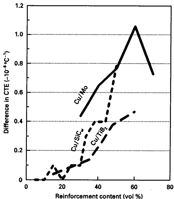
Figure 12 Variation of difference in CTE with reinforcement volume fraction between the corresponding composites made by the coated filler method and the admixture method ( \Delta \text{CTE} = \text{CTE}(\text{coated}) - \text{CTE}(\text{admixture}) ).
