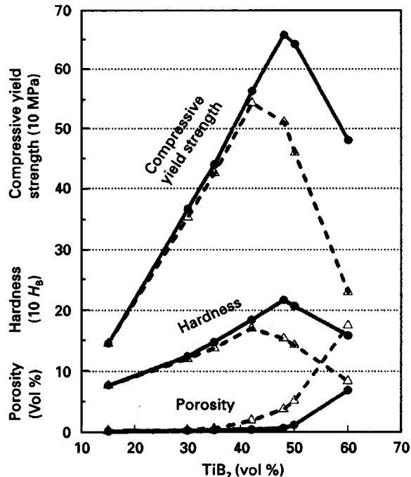
Figure 3 Variation of porosity, hardness and compressive yield strength with \text{TiB}_2 platelet volume fraction in Cu/ \text{TiB}_2 platelet composites made by the coated filler method (●) and the admixture method (Δ).
