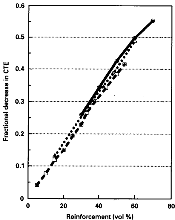
Figure 13 Variation of fractional decrease in CTE with reinforcement volume fraction of various composites made by the coated filler method. (□) Cu/SiC w ; (Δ) Cu/TiB 2 ; (○) Cu/Mo.
