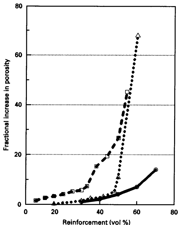
Figure 14 Variation of fractional increase in porosity with reinforcement volume fraction of various composites made by the coated filler method. (□) Cu/SiC w ; (Δ) Cu/TiB 2 ; (○) Cu/Mo.
