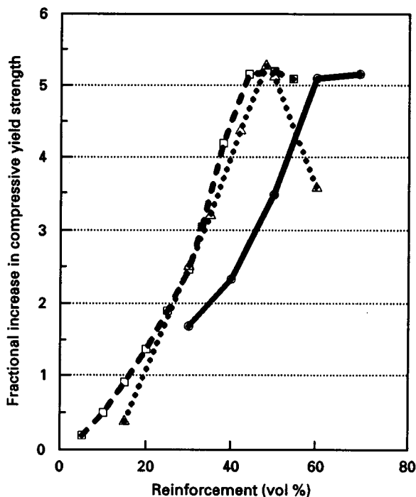
Figure 16 Variation of fractional increase in compressive yield strength with reinforcement volume fraction of various composites made by the coated filler method. (□) Cu/SiC w ; (Δ) Cu/TiB 2 ; (○) Cu/Mo.
