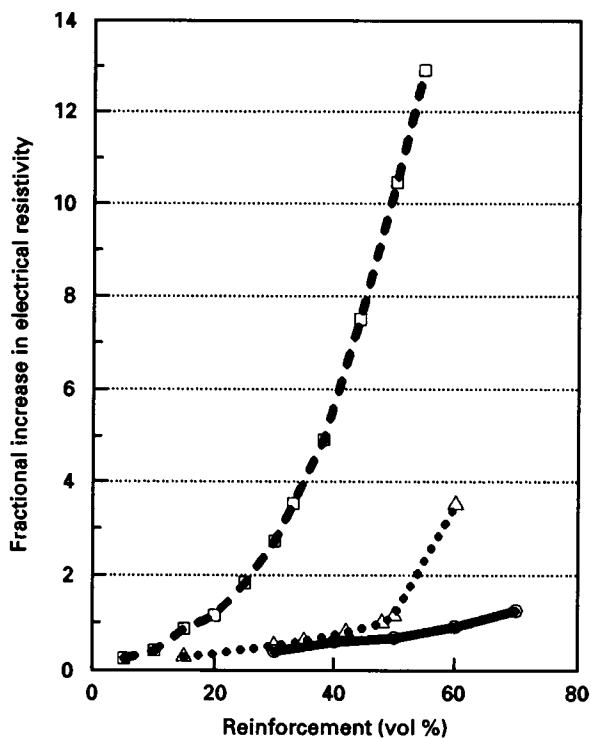
Figure 18 Variation of fractional increase in electrical resistivity with reinforcement volume fraction of various composites made by the coated filler method. (□) Cu/SiC w ; (Δ) Cu/TiB 2 ; (○) Cu/Mo.
