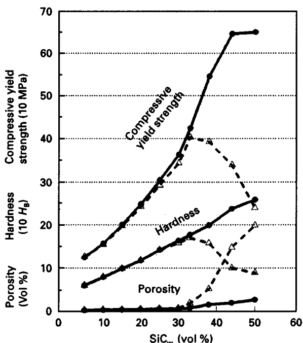
Figure 2 Variation of porosity, hardness and compressive yield strength with SiC whisker volume fraction in Cu/SiC whisker composites made by the coated filler method (●) and the admixture method (Δ).
