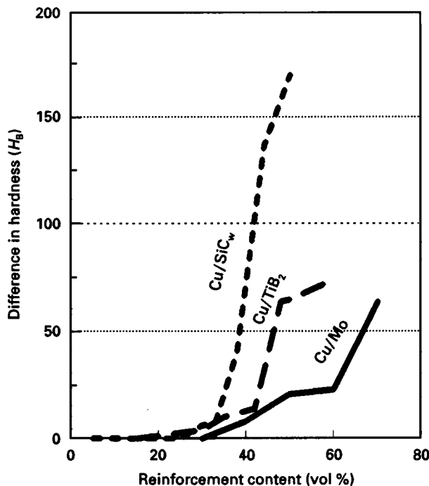
Figure 8 Variation of difference in hardness with reinforcement volume fraction between the corresponding composites made by the coated filler method and the admixture method ( \Delta H_B = H_B(\text{coated}) - H_B(\text{admixture}) ).
